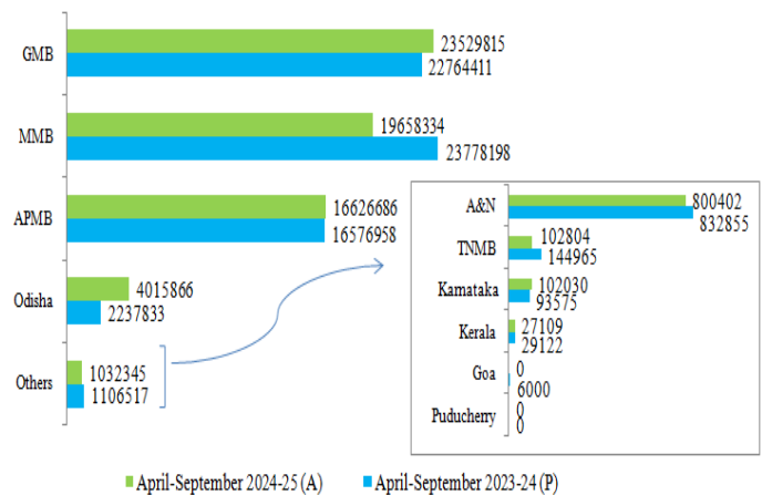
Chart 10: Coastal Cargo handled by Non-Major Ports during April-September 2024-25 vis-a-vis April-September 2023-24
